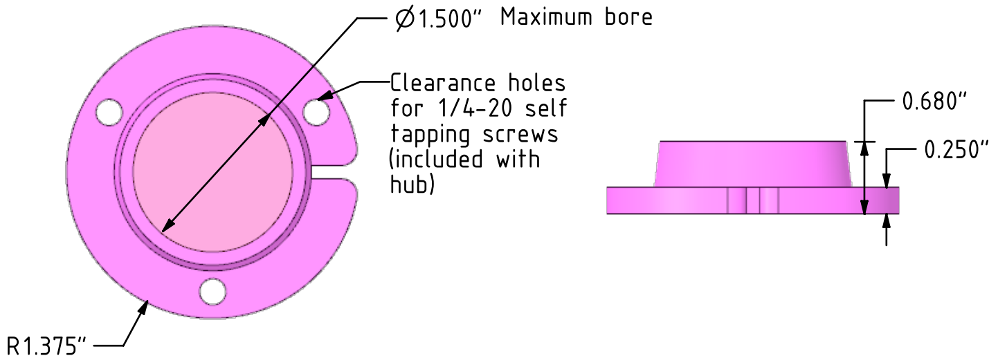
Aluminum EZE-Hub® Part# 2-00
