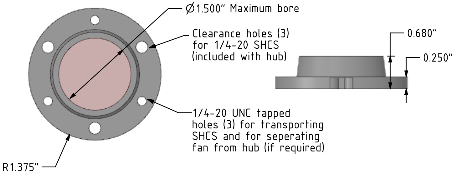
Aluminum EZE-Hub® Part# 2-00
