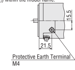
Detail Drawing of Protective Earth Terminal
