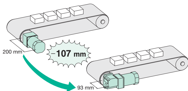
Comparison between 51K90GE-AW2J and gearhead with a gear ratio of 1:18
