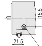
Detail Drawing of Protective Earth Terminal
